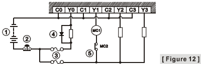
PLC Transistor output
