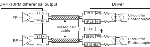
DVP-10PM differential output
