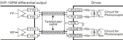
DVP-10PM differential output
