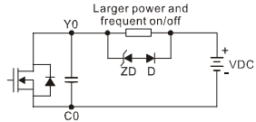
PLC Transistor output
