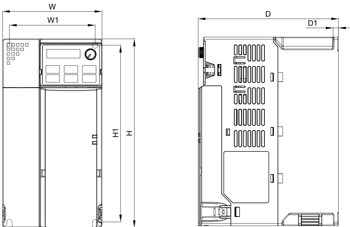
MS300 FRAME D
