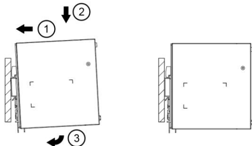
Fig. 3.1 Mounting
