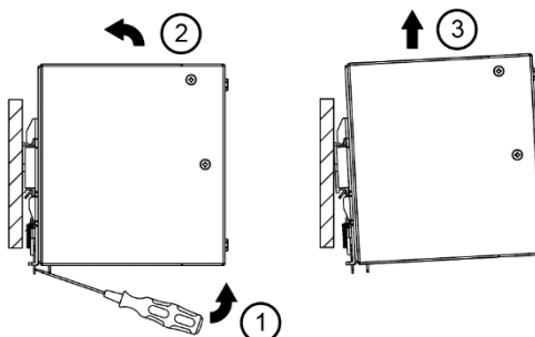
Fig. 3.2 Dismounting
