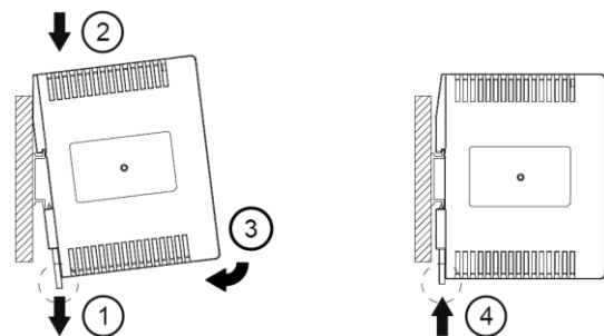
Fig. 2.1 Mounting
