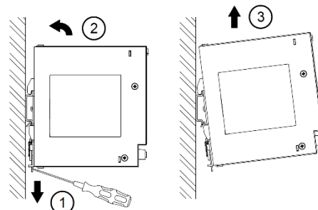
Fig. 6.2 Dismounting
