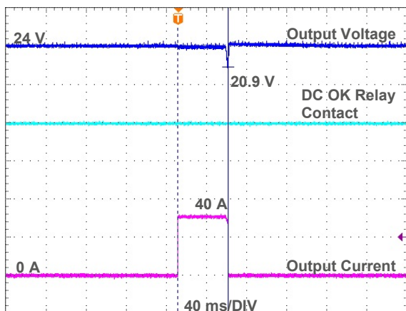
Fig. 8.1 APB 200% of nominal output current for 50 ms
