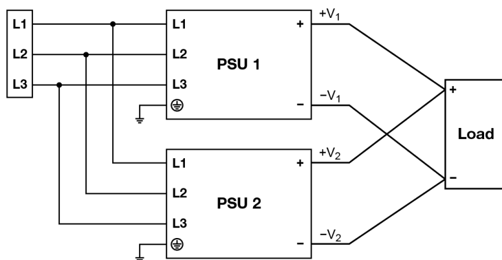
Fig. 10 Parallel Operation Connection Diagram
