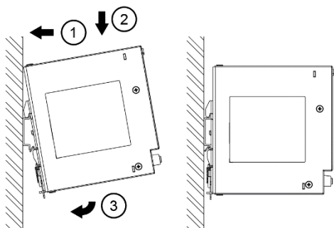
Fig. 7.1 Mounting
