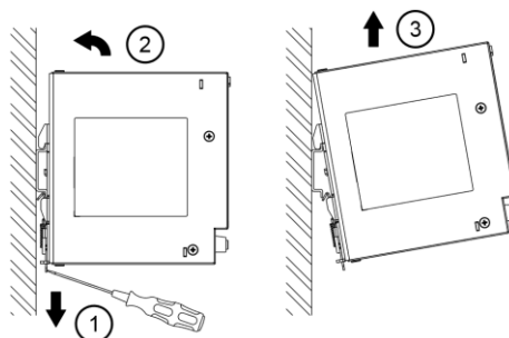
Fig. 7.2 Dismounting
