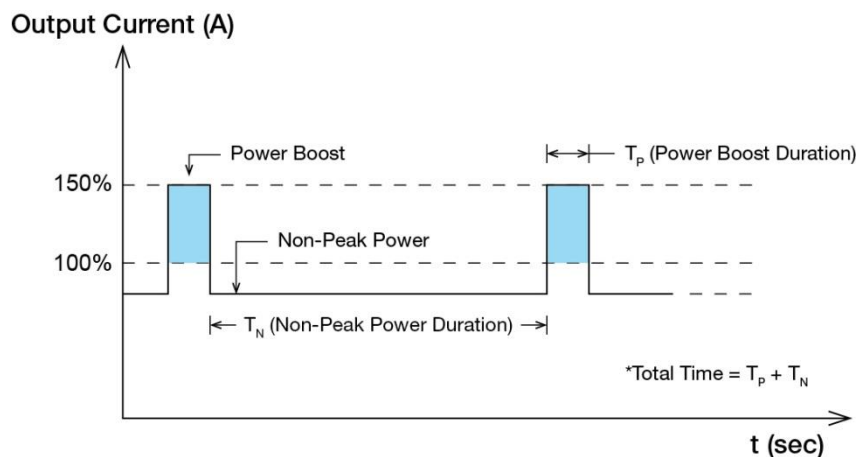
Fig. 8 Duty Cycle Calculation
