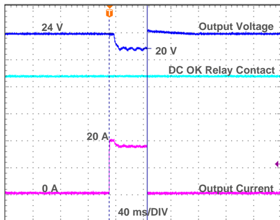
Fig. 9 APB 200% of nominal output current for 50 ms
