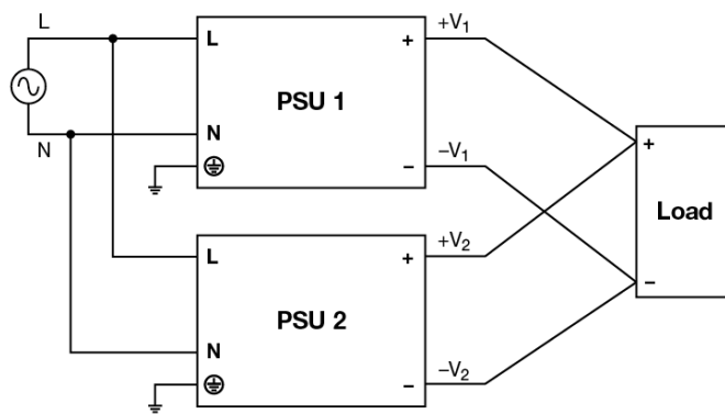
Fig. 11 Parallel Operation Connection Diagram
