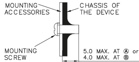
Fig. 4 Assembly Reference
